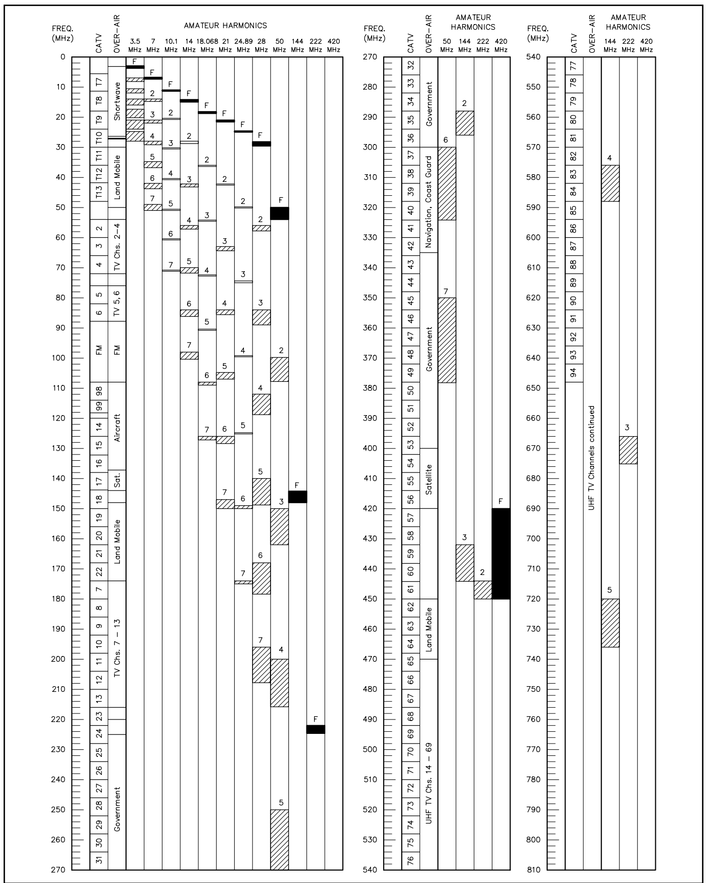
Figure 6.2. This chart shows CATV and broadcast channels used in the United States. The frequency relationship to the harmonics of HF, VHF and UHF amateur bands can be readily seen. This will help identify those channels that are harmonically related to the transmit frequency. Use this chart to determine if there is a harmonic relationship between operating frequency and any TV channels affected by station operation. If the interference is only on channels that are multiples of your operating frequency, you clearly have interference from harmonics. (It is not certain that these harmonics are coming from your station, however.)
