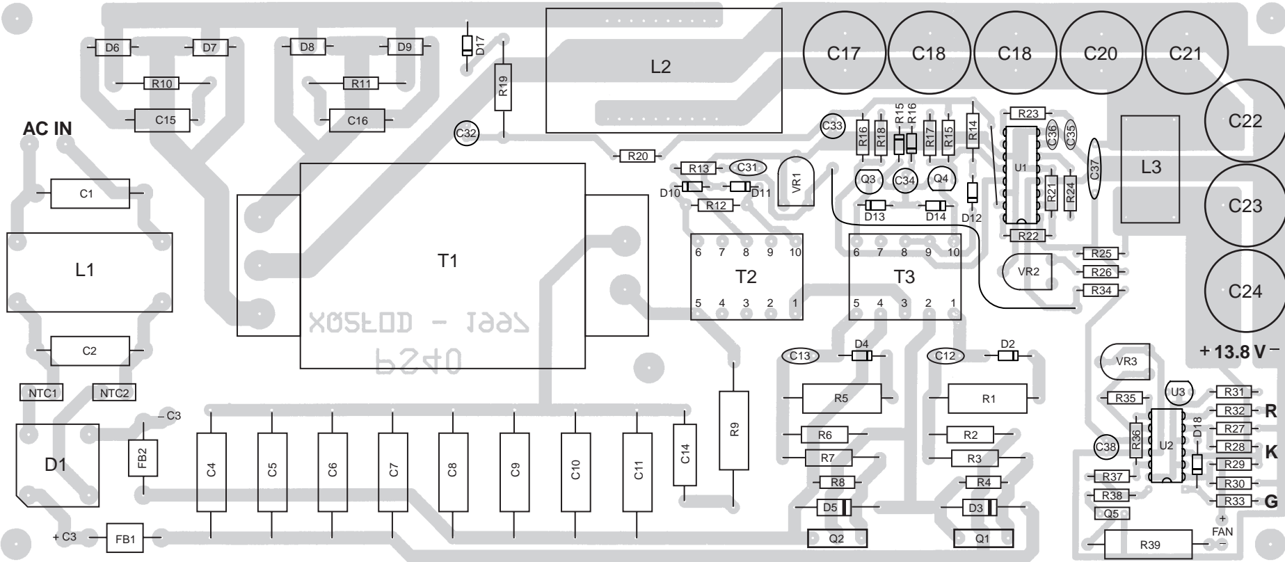
A 13.8-V, 40-A Switching Power Supply, Chapter 11
