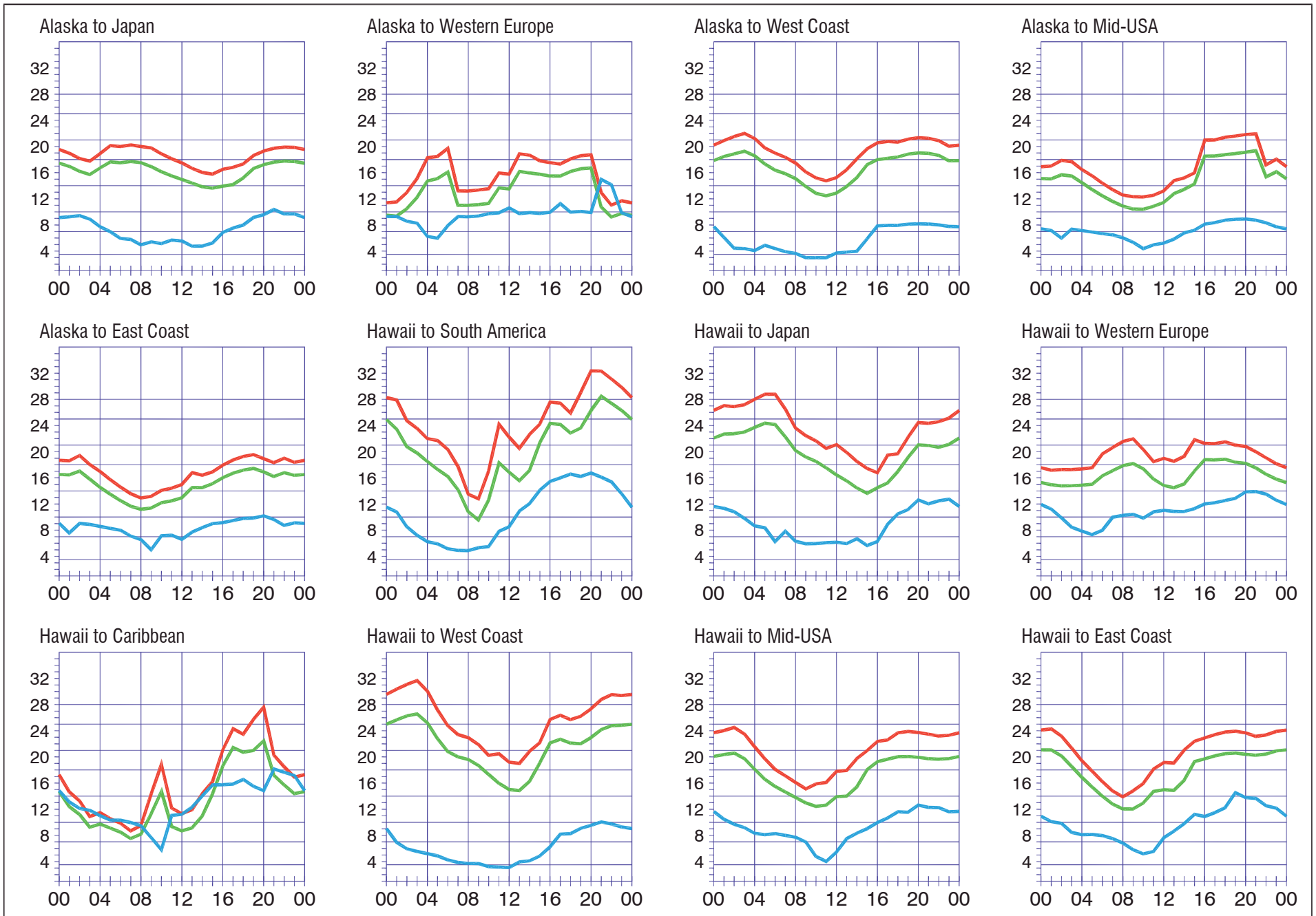
When are the bands open? These charts, generated using CAPman, show probabilities for average HF propagation in the month of July 2004 for the paths indicated. The horizontal axes show Coordinated Universal Time (UTC), and the vertical axes frequency in MHz. On 10 % of the days of this period, the highest frequencies propagated will be at least as high as the upper red curves (HPF, highest possible frequency) and on 50 % of the days they will be at least as high as the green curves (MUF, classical maximum usable frequency). The blue curves show the lowest usable frequency (LUF) for a 1500-W CW transmitter. For SSB or a lower transmitter power, the LUF will be somewhat higher than the blue curves indicate. See Oct 1994 QST, pp 27-30, and Feb 1995 QST, pp 34-36, for more details. The predictions assume an observed 2800-MHz solar flux value of 94. This is a Low level of solar activity. See the detailed propagation tables on The ARRL Antenna Book CD-ROM.
