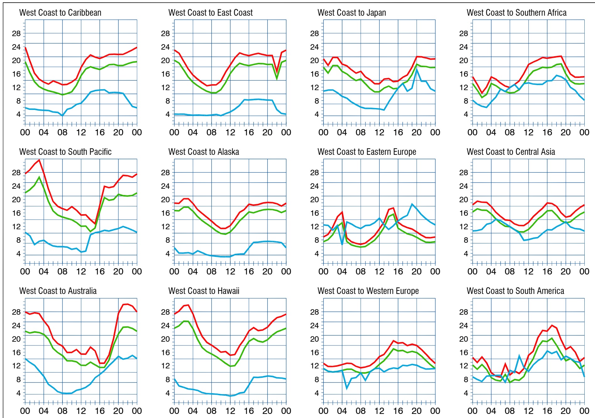
When are the bands open? These charts, generated using CAPman, show probabilities for average HF propagation in the month of August 2008 for the paths indicated. The horizontal axes show Coordinated Universal Time (UTC), and the vertical axes frequency in MHz. On 10% of the days of this period, the highest frequencies propagated will be at least as high as the upper red curves (HPF, highest possible frequency) and on 50% of the days they will be at least as high as the green curves (MUF, classical maximum usable frequency). The blue curves show the lowest usable frequency (LUF) for a 1500-W CW transmitter. For SSB or a lower transmitter power, the LUF will be somewhat higher than the blue curves indicate. See Oct 1994 QST , pp 27-30, and Feb 1995 QST , pp 34-36, for more details. The predictions assume an observed 2800-MHz solar flux value of 68. This is a Very Low level of solar activity. See the detailed propagation tables on The ARRL Antenna Book CD-ROM .
