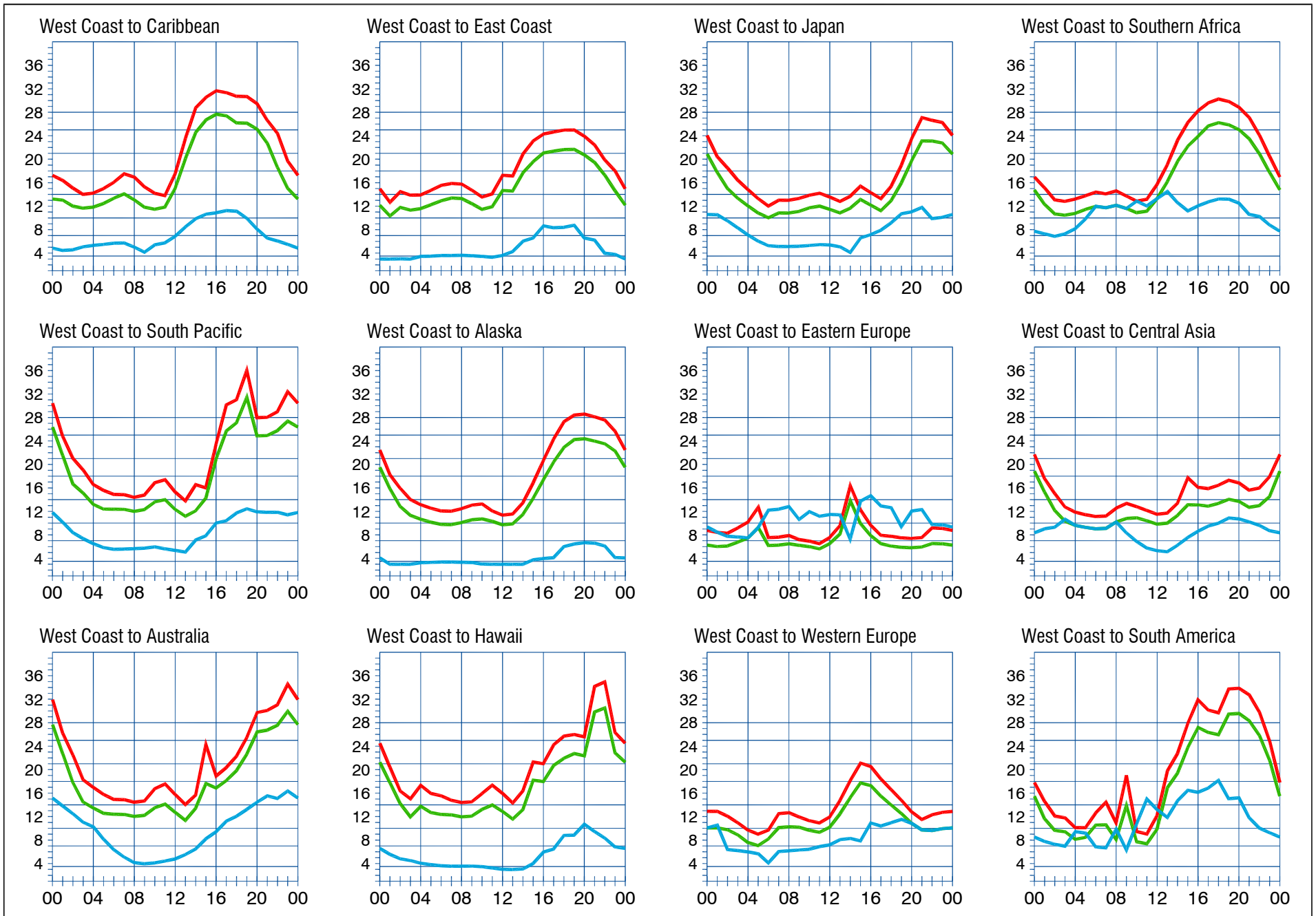
When are the bands open? These charts, generated using CAPman, show probabilities for average HF propagation in the month of November 2008 for the paths indicated. The horizontal axes show Coordinated Universal Time (UTC), and the vertical axes frequency in MHz. On 10% of the days of this period, the highest frequencies propagated will be at least as high as the upper red curves (HPF, highest possible frequency) and on 50% of the days they will be at least as high as the green curves (MUF, classical maximum usable frequency). The blue curves show the lowest usable frequency (LUF) for a 1500-W CW transmitter. For SSB or a lower transmitter power, the LUF will be somewhat higher than the blue curves indicate. See Oct 1994 QST , pp 27-30, and Feb 1995 QST , pp 34-36, for more details. The predictions assume an observed 2800-MHz solar flux value of 71. This is a Very Low level of solar activity. See the detailed propagation tables on The ARRL Antenna Book CD-ROM .
