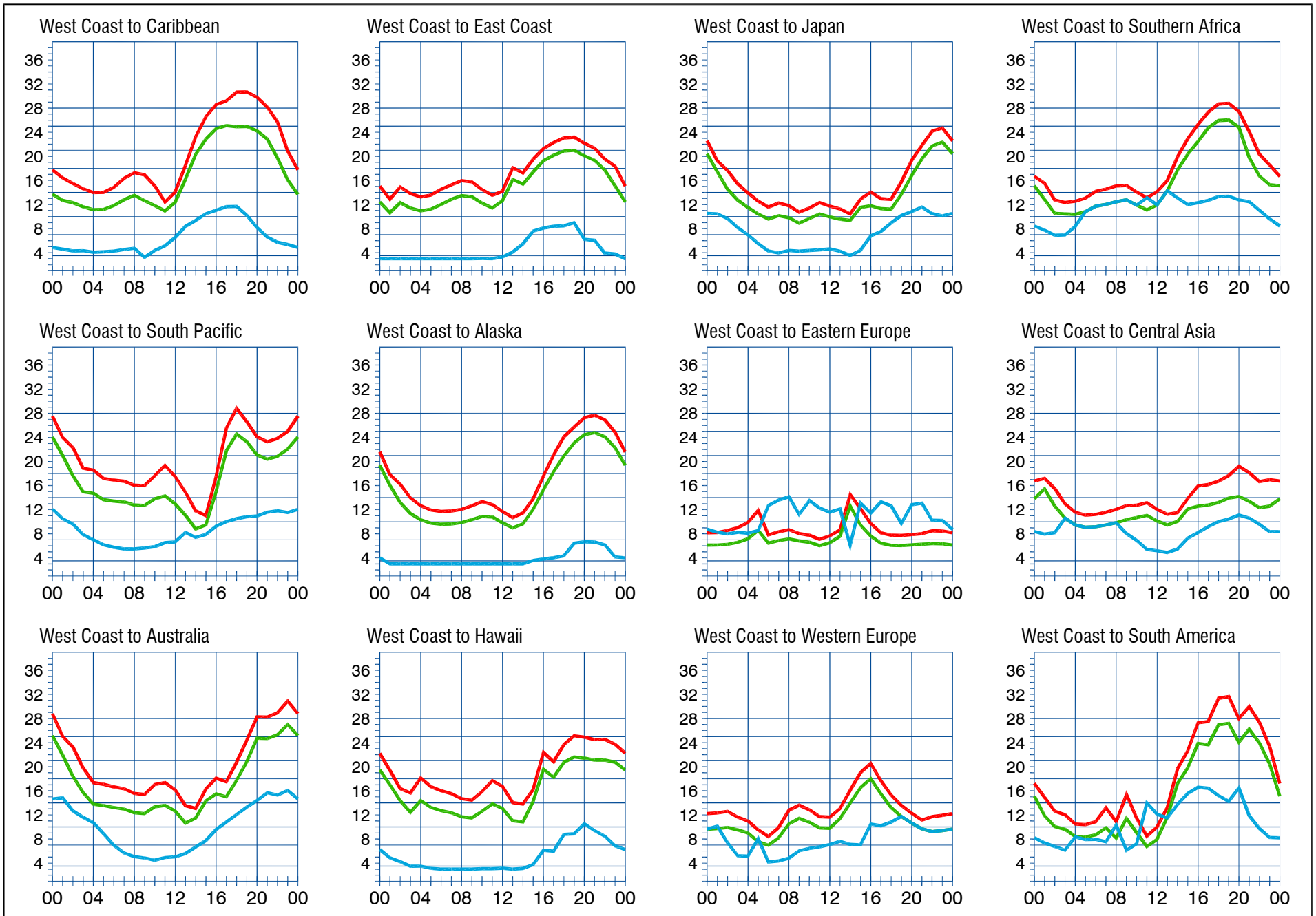
When are the bands open? These charts, generated using CAPman, show probabilities for average HF propagation in the month of January 2009 for the paths indicated. The horizontal axes show Coordinated Universal Time (UTC), and the vertical axes frequency in MHz. On 10% of the days of this period, the highest frequencies propagated will be at least as high as the upper red curves (HPF, highest possible frequency) and on 50% of the days they will be at least as high as the green curves (MUF, classical maximum usable frequency). The blue curves show the lowest usable frequency (LUF) for a 1500-W CW transmitter. For SSB or a lower transmitter power, the LUF will be somewhat higher than the blue curves indicate. See Oct 1994 QST , pp 27-30, and Feb 1995 QST , pp 34-36, for more details. The predictions assume an observed 2800-MHz solar flux value of 75. This is a Very Low level of solar activity. See the detailed propagation tables on The ARRL Antenna Book CD-ROM .
