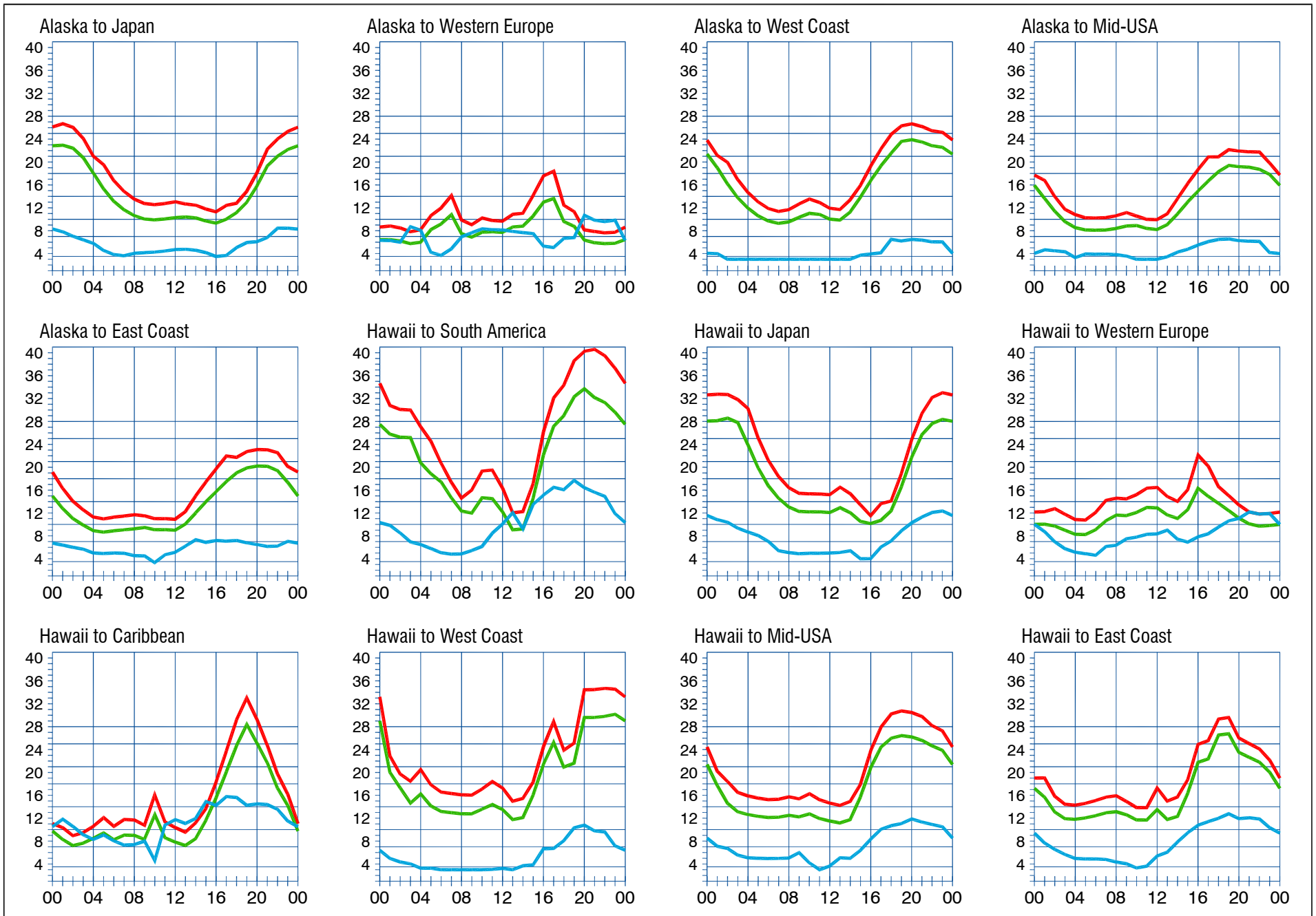
When are the bands open? These charts, generated using CAPman, show probabilities for average HF propagation in the month of February 2009 for the paths indicated. The horizontal axes show Coordinated Universal Time (UTC), and the vertical axes frequency in MHz. On 10% of the days of this period, the highest frequencies propagated will be at least as high as the upper red curves (HPF, highest possible frequency) and on 50% of the days they will be at least as high as the green curves (MUF, classical maximum usable frequency). The blue curves show the lowest usable frequency (LUF) for a 1500-W CW transmitter. For SSB or a lower transmitter power, the LUF will be somewhat higher than the blue curves indicate. See Oct 1994 QST , pp 27-30, and Feb 1995 QST , pp 34-36, for more details. The predictions assume an observed 2800-MHz solar flux value of 77. This is a Very Low level of solar activity. See the detailed propagation tables on The ARRL Antenna Book CD-ROM .
