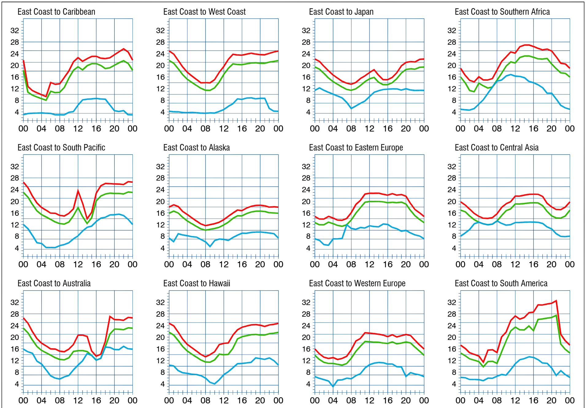
When are the bands open? These charts, generated using CAPman, show probabilities for average HF propagation in the month of August 2009 for the paths indicated. The horizontal axes show Coordinated Universal Time (UTC), and the vertical axes frequency in MHz. On 10% of the days of this period, the highest frequencies propagated will be at least as high as the upper red curves (HPF, highest possible frequency) and on 50% of the days they will be at least as high as the green curves (MUF, classical maximum usable frequency). The blue curves show the lowest usable frequency (LUF) for a 1500-W CW transmitter. For SSB or a lower transmitter power, the LUF will be somewhat higher than the blue curves indicate. See Oct 1994 QST , pp 27-30, and Feb 1995 QST , pp 34-36, for more details. The predictions assume an observed 2800-MHz solar flux value of 92. This is a Low level of solar activity. See the detailed propagation tables on The ARRL Antenna Book CD-ROM .
