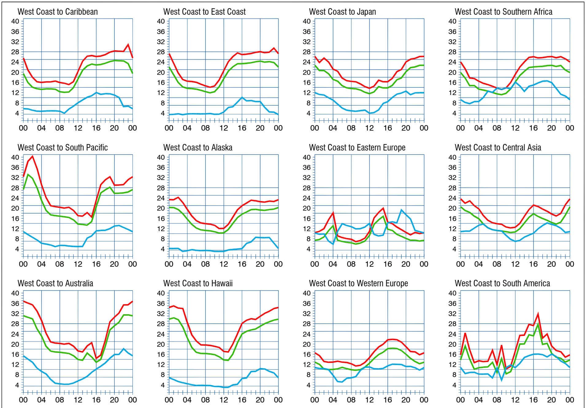
When are the bands open? These charts, generated using CAPman, show probabilities for average HF propagation in the month of September 2009 for the paths indicated. The horizontal axes show Coordinated Universal Time (UTC), and the vertical axes frequency in MHz. On 10% of the days of this period, the highest frequencies propagated will be at least as high as the upper red curves (HPF, highest possible frequency) and on 50% of the days they will be at least as high as the green curves (MUF, classical maximum usable frequency). The blue curves show the lowest usable frequency (LUF) for a 1500-W CW transmitter. For SSB or a lower transmitter power, the LUF will be somewhat higher than the blue curves indicate. See Oct 1994 QST , pp 27-30, and Feb 1995 QST , pp 34-36, for more details. The predictions assume an observed 2800-MHz solar flux value of 95. This is a Medium level of solar activity. See the detailed propagation tables on The ARRL Antenna Book CD-ROM .
