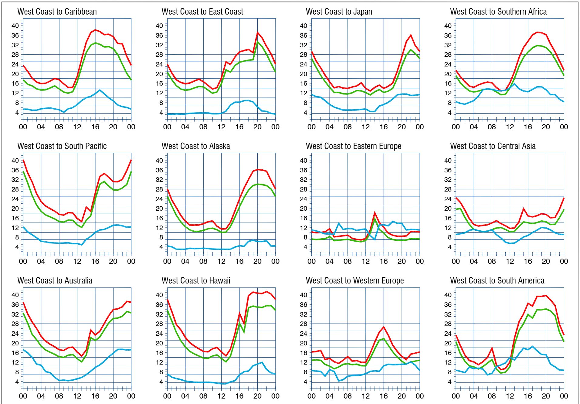
When are the bands open? These charts, generated using CAPman, show probabilities for average HF propagation in the month of November 2009 for the paths indicated. The horizontal axes show Coordinated Universal Time (UTC), and the vertical axes frequency in MHz. On 10% of the days of this period, the highest frequencies propagated will be at least as high as the upper red curves (HPF, highest possible frequency) and on 50% of the days they will be at least as high as the green curves (MUF, classical maximum usable frequency). The blue curves show the lowest usable frequency (LUF) for a 1500-W CW transmitter. For SSB or a lower transmitter power, the LUF will be somewhat higher than the blue curves indicate. See Oct 1994 QST , pp 27-30, and Feb 1995 QST , pp 34-36, for more details. The predictions assume an observed 2800-MHz solar flux value of 101. This is a Medium level of solar activity. See the detailed propagation tables on The ARRL Antenna Book CD-ROM .
