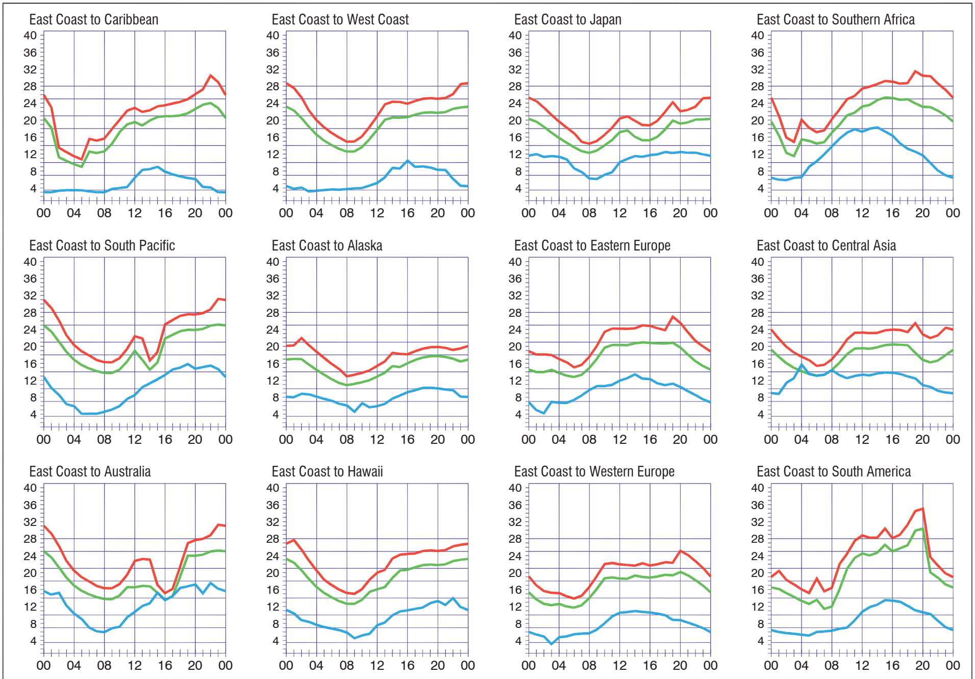
When are the bands open? These charts, generated using CAPman, show probabilities for average HF propagation in the month of May 2004 for the paths indicated. The horizontal axes show Coordinated Universal Time (UTC), and the vertical axes frequency in MHz. On 10 % of the days of this period, the highest frequencies propagated will be at least as high as the upper red curves (HPF, highest possible frequency) and on 50 % of the days they will be at least as high as the green curves (MUF, classical maximum usable frequency). The blue curves show the lowest usable frequency (LUF) for a 1500-W CW transmitter. For SSB or a lower transmitter power, the LUF will be somewhat higher than the blue curves indicate. See Oct 1994 QST , pp 27-30, and Feb 1995 QST , pp 34-36, for more details. The predictions assume an observed 2800-MHz solar flux value of 98. This is a Medium level of solar activity. See the detailed propagation tables on The ARRL Antenna Book CD-ROM .
