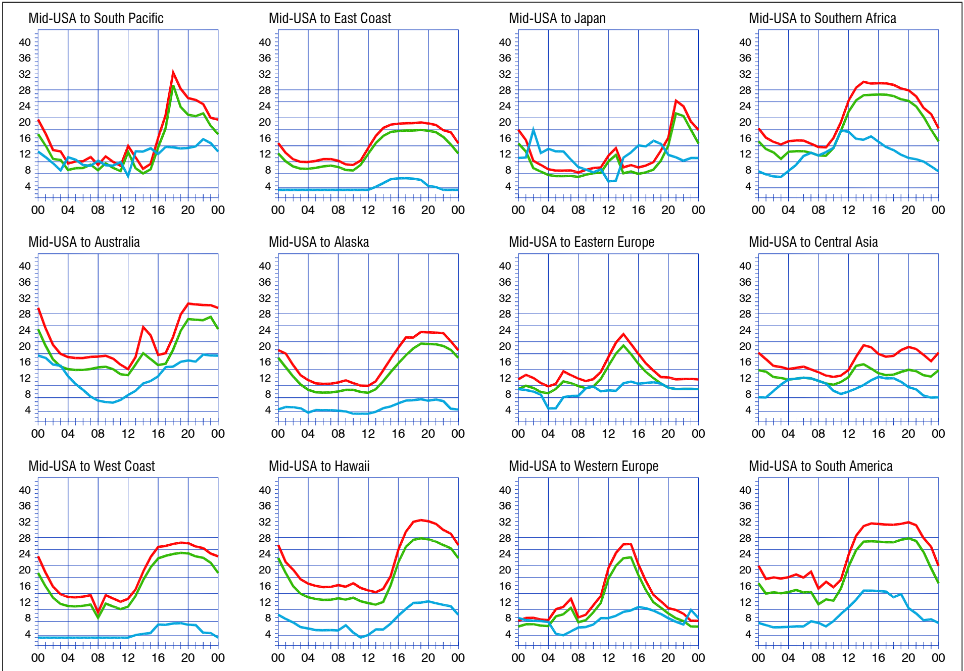
When are the bands open? These charts, generated using CAPman, show probabilities for average HF propagation in the month of February 2005 for the paths indicated. The horizontal axes show Coordinated Universal Time (UTC), and the vertical axes frequency in MHz. On 10% of the days of this period, the highest frequencies propagated will be at least as high as the upper red curves (HPF, highest possible frequency) and on 50% of the days they will be at least as high as the green curves (MUF, classical maximum usable frequency). The blue curves show the lowest usable frequency (LUF) for a 1500-W CW transmitter. For SSB or a lower transmitter power, the LUF will be somewhat higher than the blue curves indicate. See Oct 1994 QST , pp 27-30, and Feb 1995 QST , pp 34-36, for more details. The predictions assume an observed 2800-MHz solar flux value of 85. This is a Low level of solar activity. See the detailed propagation tables on The ARRL Antenna Book CD-ROM .
