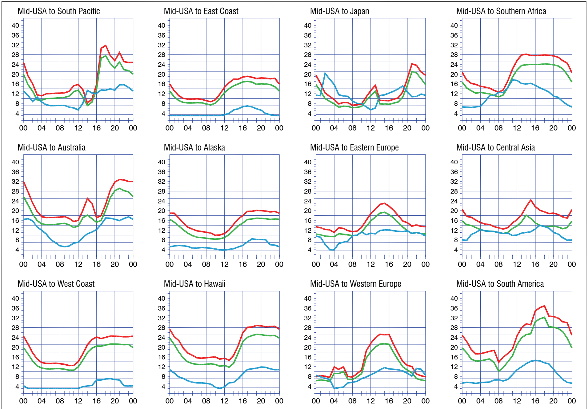
When are the bands open? These charts, generated using CAPman, show probabilities for average HF propagation in the month of March 2005 for the paths indicated. The horizontal axes show Coordinated Universal Time (UTC), and the vertical axes frequency in MHz. On 10% of the days of this period, the highest frequencies propagated will be at least as high as the upper red curves (HPF, highest possible frequency) and on 50% of the days they will be at least as high as the green curves (MUF, classical maximum usable frequency). The blue curves show the lowest usable frequency (LUF) for a 1500-W CW transmitter. For SSB or a lower transmitter power, the LUF will be somewhat higher than the blue curves indicate. See Oct 1994 QST , pp 27-30, and Feb 1995 QST , pp 34-36, for more details. The predictions assume an observed 2800-MHz solar flux value of 84. This is a Low level of solar activity. See the detailed propagation tables on The ARRL Antenna Book CD-ROM .
