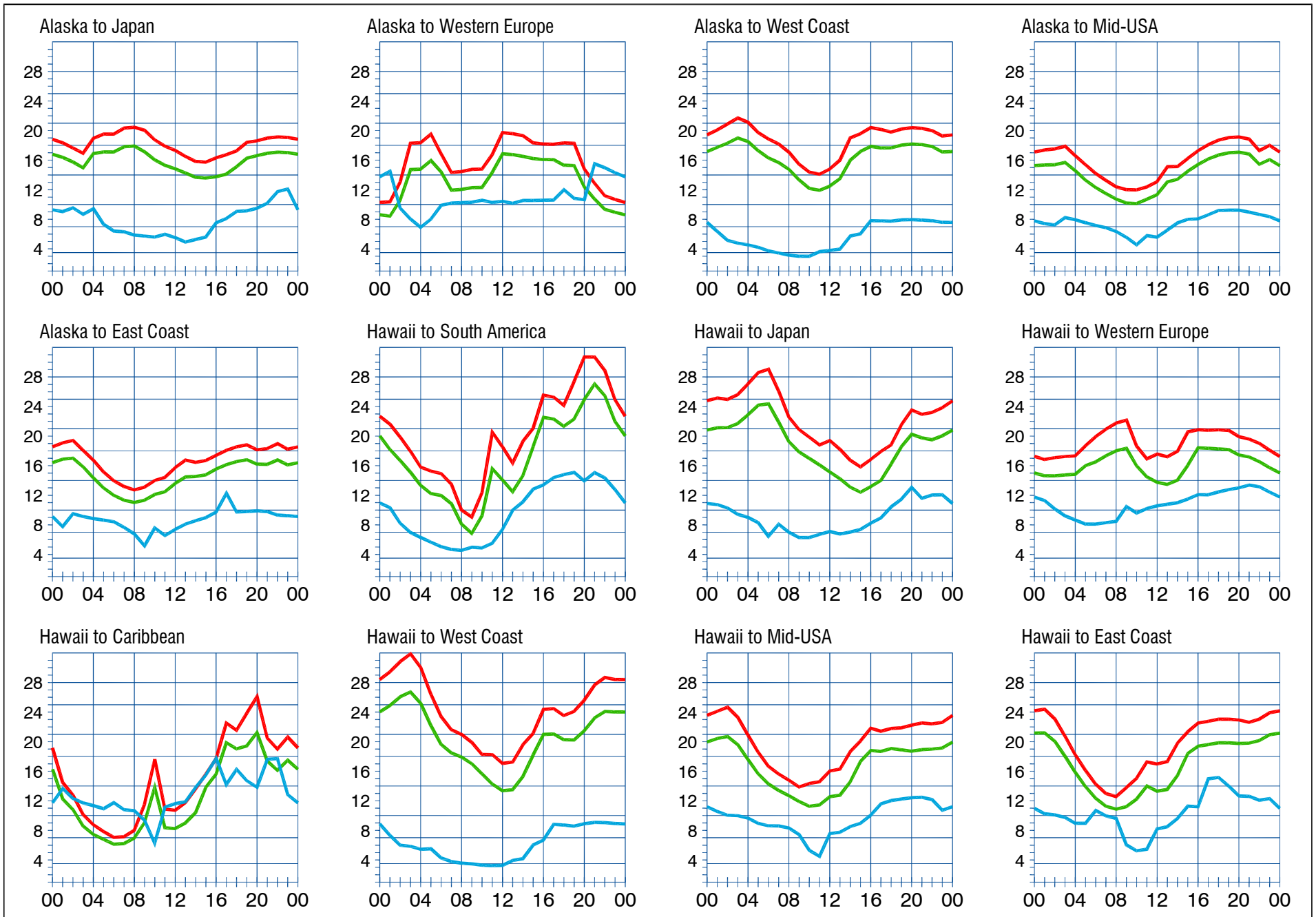
When are the bands open? These charts, generated using CAPman, show probabilities for average HF propagation in the month of June 2008 for the paths indicated. The horizontal axes show Coordinated Universal Time (UTC), and the vertical axes frequency in MHz. On 10% of the days of this period, the highest frequencies propagated will be at least as high as the upper red curves (HPF, highest possible frequency) and on 50% of the days they will be at least as high as the green curves (MUF, classical maximum usable frequency). The blue curves show the lowest usable frequency (LUF) for a 1500-W CW transmitter. For SSB or a lower transmitter power, the LUF will be somewhat higher than the blue curves indicate. See Oct 1994 QST , pp 27-30, and Feb 1995 QST , pp 34-36, for more details. The predictions assume an observed 2800-MHz solar flux value of 66. This is a Very Low level of solar activity. See the detailed propagation tables on The ARRL Antenna Book CD-ROM .
