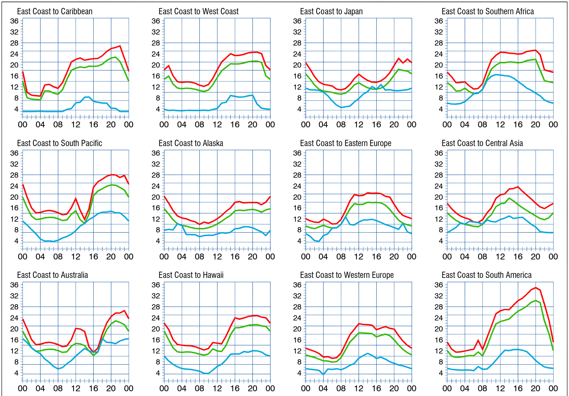
When are the bands open? These charts, generated using CAPman, show probabilities for average HF propagation in the month of September 2008 for the paths indicated. The horizontal axes show Coordinated Universal Time (UTC), and the vertical axes frequency in MHz. On 10% of the days of this period, the highest frequencies propagated will be at least as high as the upper red curves (HPF, highest possible frequency) and on 50% of the days they will be at least as high as the green curves (MUF, classical maximum usable frequency). The blue curves show the lowest usable frequency (LUF) for a 1500-W CW transmitter. For SSB or a lower transmitter power, the LUF will be somewhat higher than the blue curves indicate. See Oct 1994 QST , pp 27-30, and Feb 1995 QST , pp 34-36, for more details. The predictions assume an observed 2800-MHz solar flux value of 69. This is a Very Low level of solar activity. See the detailed propagation tables on The ARRL Antenna Book CD-ROM .
