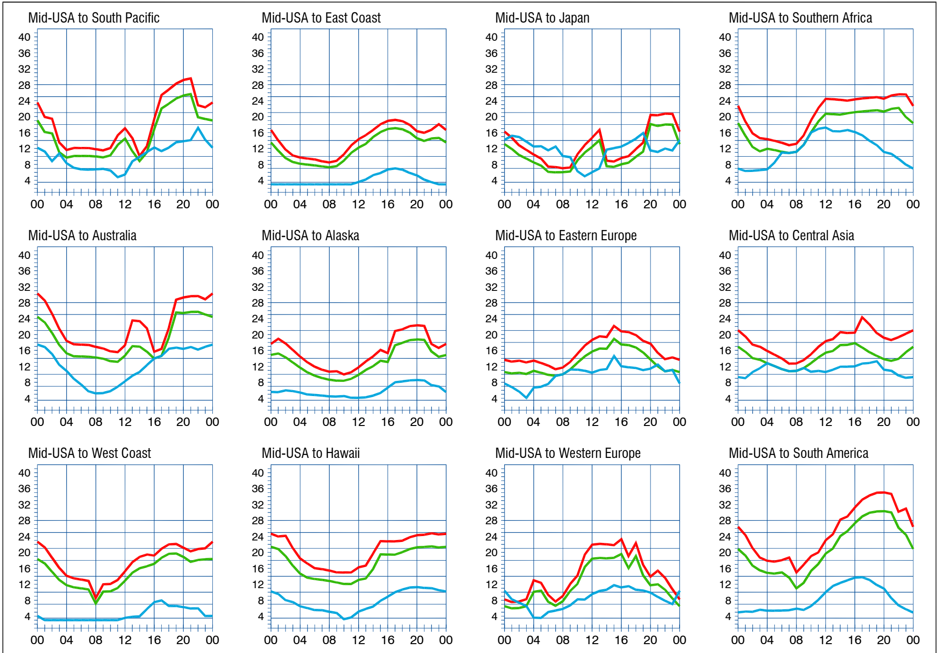
When are the bands open? These charts, generated using CAPman, show probabilities for average HF propagation in the month of April 2009 for the paths indicated. The horizontal axes show Coordinated Universal Time (UTC), and the vertical axes frequency in MHz. On 10% of the days of this period, the highest frequencies propagated will be at least as high as the upper red curves (HPF, highest possible frequency) and on 50% of the days they will be at least as high as the green curves (MUF, classical maximum usable frequency). The blue curves show the lowest usable frequency (LUF) for a 1500-W CW transmitter. For SSB or a lower transmitter power, the LUF will be somewhat higher than the blue curves indicate. See Oct 1994 QST , pp 27-30, and Feb 1995 QST , pp 34-36, for more details. The predictions assume an observed 2800-MHz solar flux value of 81. This is a Low level of solar activity. See the detailed propagation tables on The ARRL Antenna Book CD-ROM .
